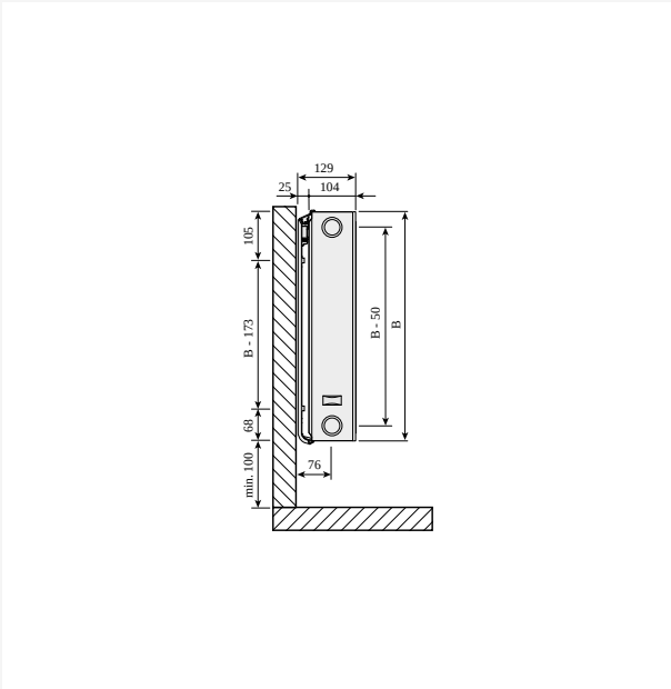
DimensionalDrawing - Plan Compact, type 22, side view with Monclac wall brackets
