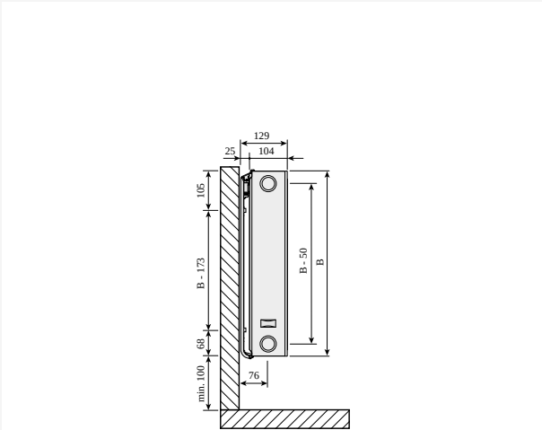
DimensionalDrawing - Plan Compact - table
