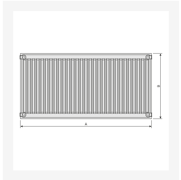
DimensionalDrawing - 1.2 PR-Plan-Hygiene-RV-T10-0924
