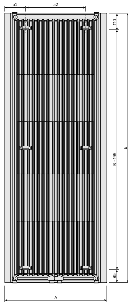
DimensionalDrawing - New_Paros V rear view
