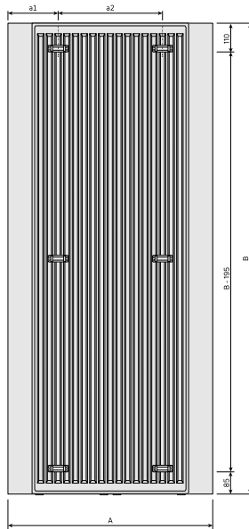
DimensionalDrawing - New_Paros V rear view
