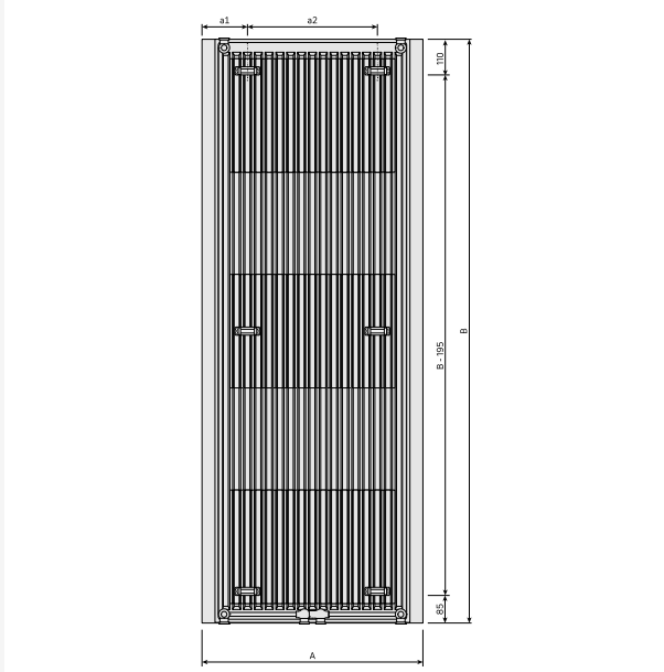
DimensionalDrawing - New_Paros V rear view
