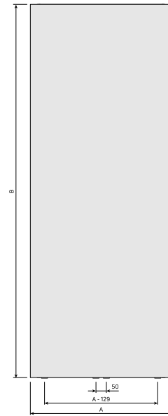
DimensionalDrawing - New_Paros V front view
