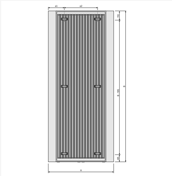
DimensionalDrawing - New_Paros V rear view
