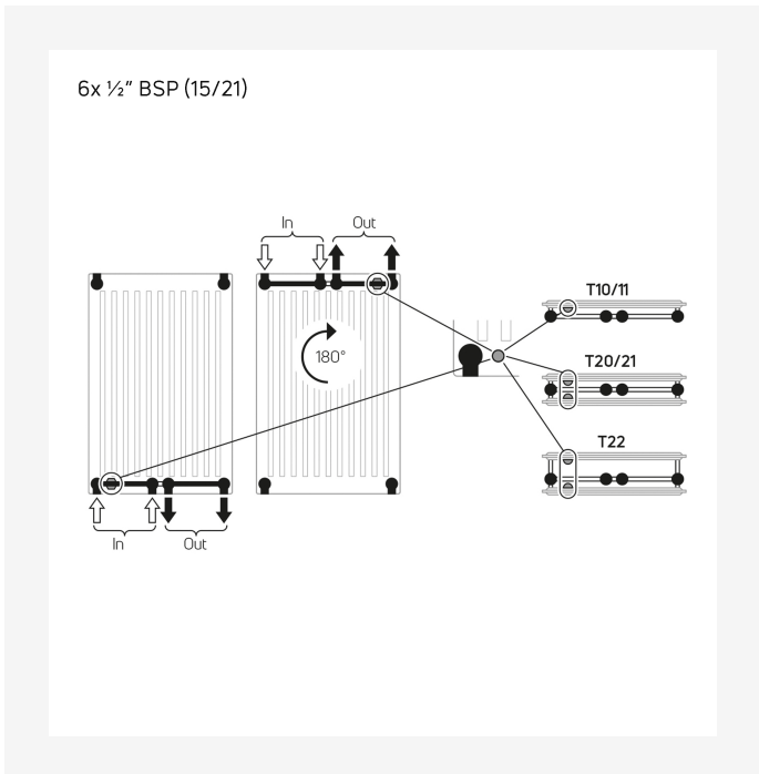
Installation - MysonPlanVerticalPlanPlusVertical-TechnicalDrawing-ConnectionOptions-2000x2000
