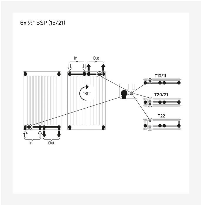
Installation - MysonPlanVerticalPlanPlusVertical- TechnicalDrawing-ConnectionOptions-2000x2000
