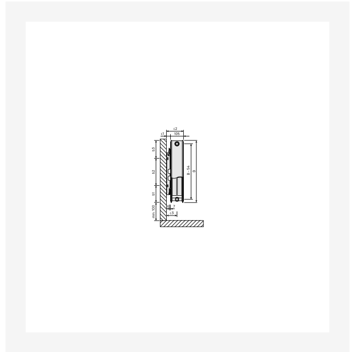
DimensionalDrawing - Reggane 3010 Compact, type 22 H400_900, Vue latérale
