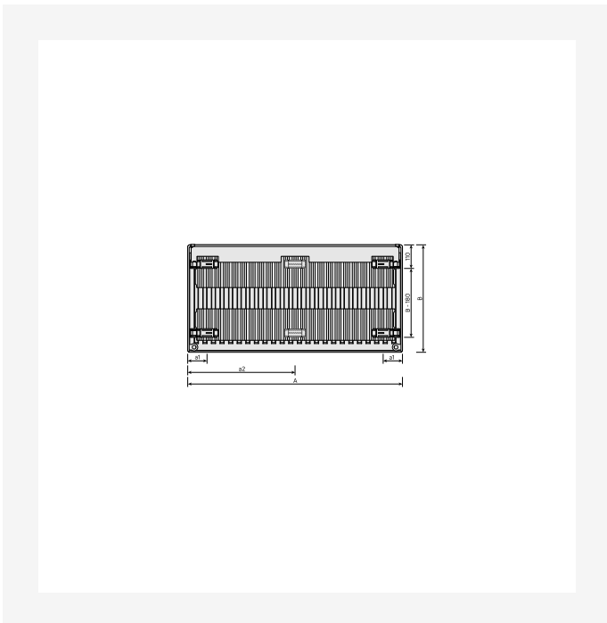
DimensionalDrawing - Reggane 3010 Compact, type 11, Vue arrière
