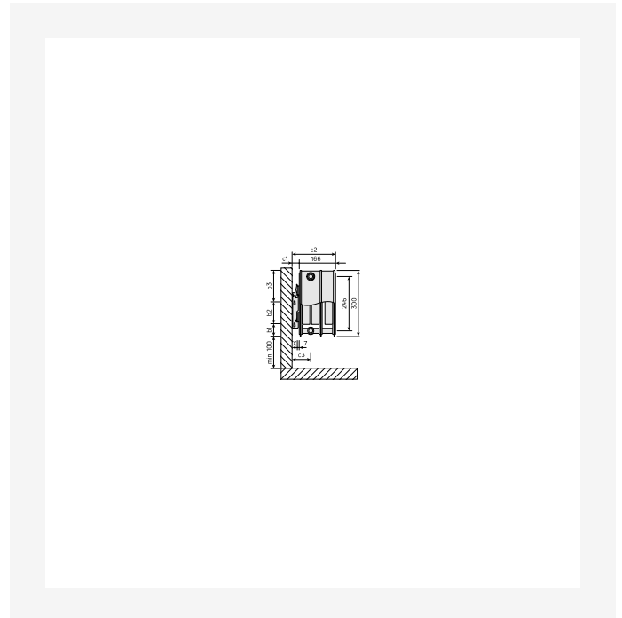
DimensionalDrawing - Reggane 3010 Compact, type 33, Vue latérale
