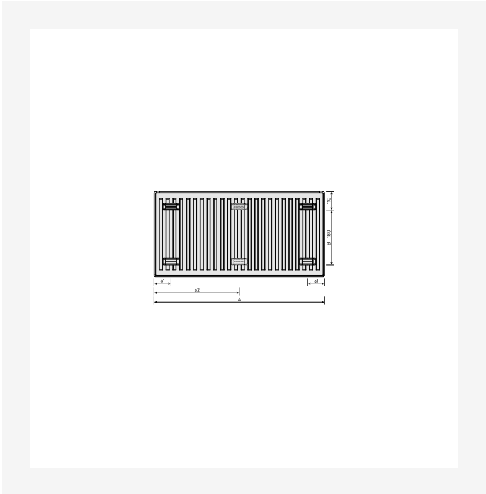
DimensionalDrawing - Reggane 3010 Compact, type 21, 22, 33, Vue arrière
