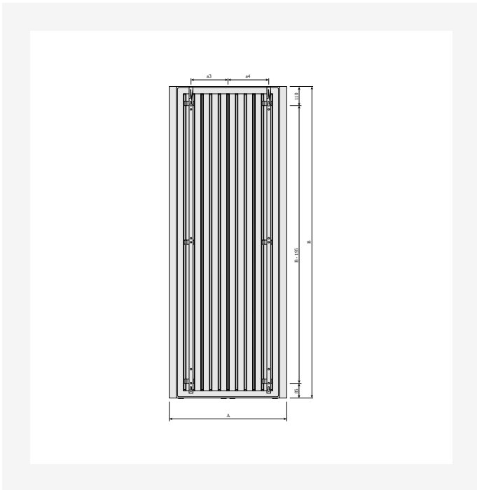
Dimensional Drawing - PR-PAV-BV-MCW-V-0721
