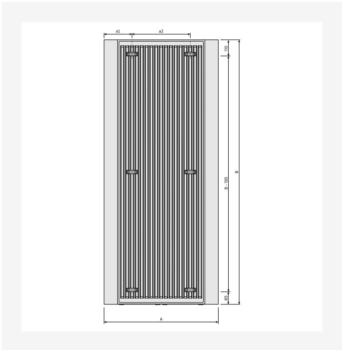
Dimensional Drawing - New_Paros V_RV_T21_0124
