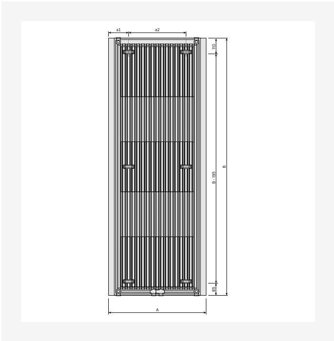
Dimensional Drawing - New_Paros V_RV_T11_0124
