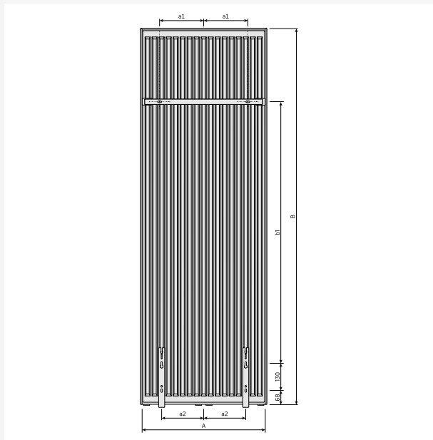
DimensionalDrawing - Kos V / Faro V, takaa
