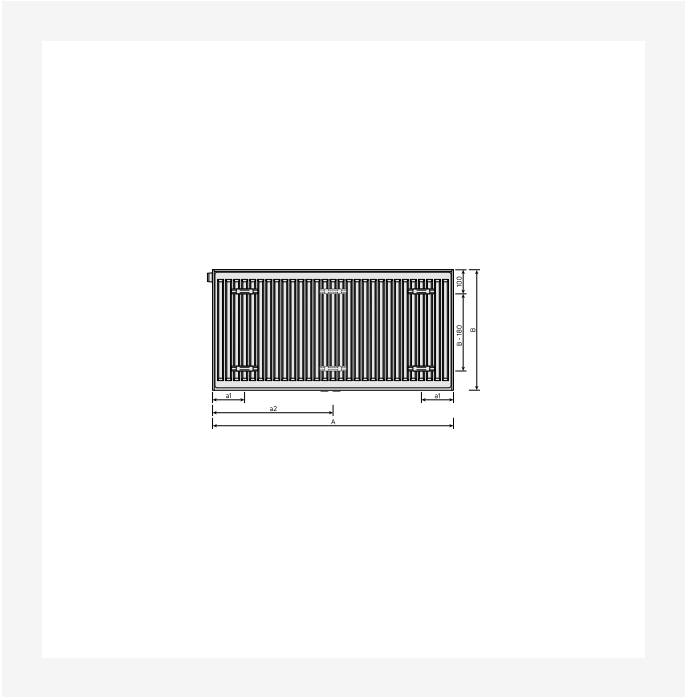
DimensionalDrawing - Flex, tyytit 21, 22, 33, takaa
