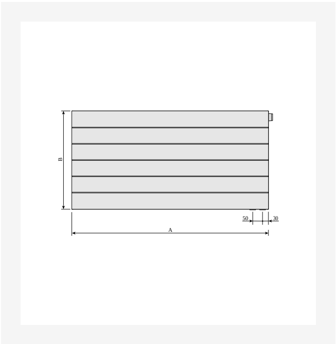
DimensionalDrawing - Ramo Ventil Compact, eestvaade, parem
