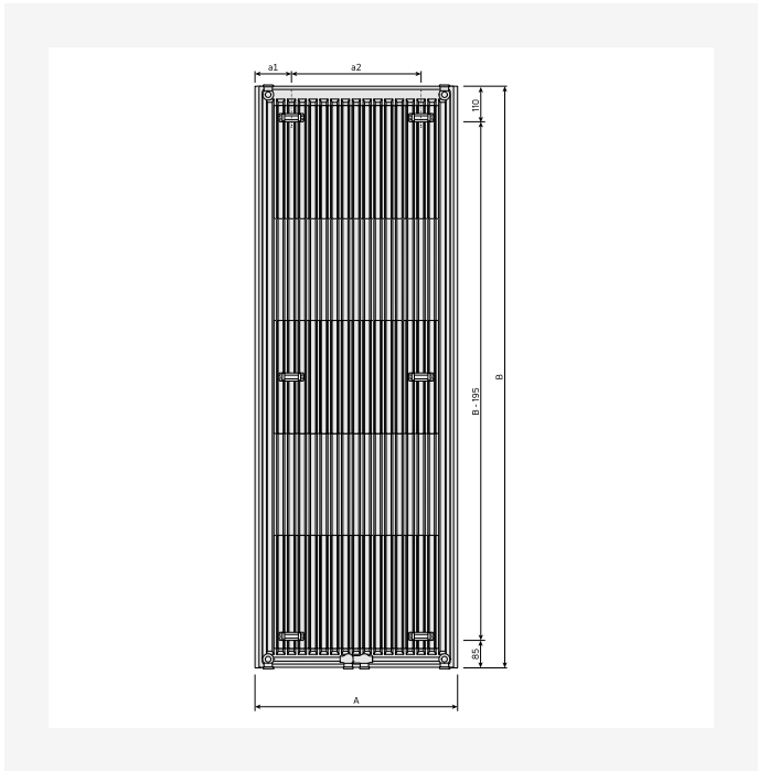
DimensionalDrawing - Tinos V, type 11, bagfra
