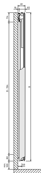
DimensionalDrawing - Tinos V / Paros V, type 11, sidevisning
