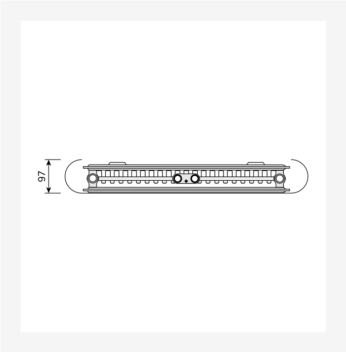
DimensionalDrawing - Paros V, type 21, set oppefra
