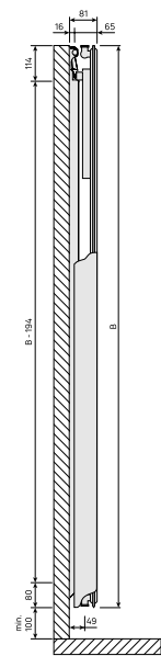
DimensionalDrawing - Tinos V / Paros V, type 11, sidevisning
