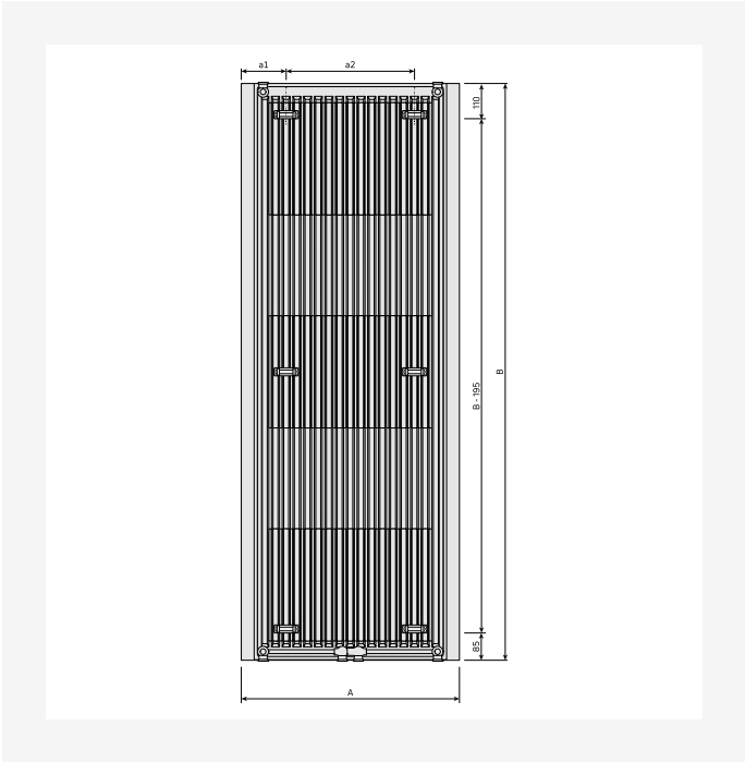
DimensionalDrawing - Paros V, type 11, bagfra
