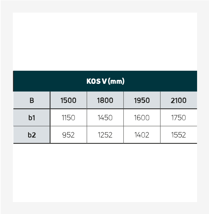
DimensionalDrawing - Kos V, Faro V - table B
